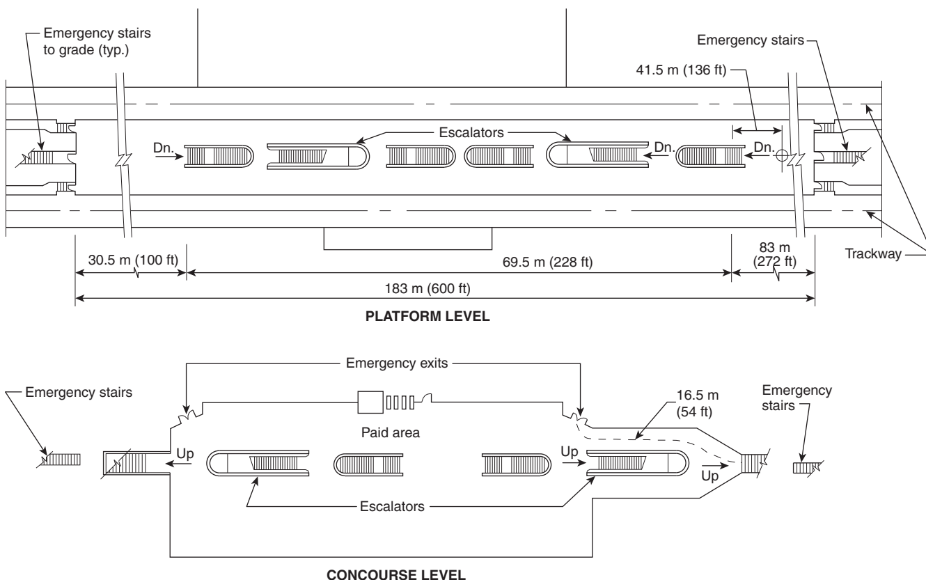
FIGURE C.1.3 Center-Platform Station.
