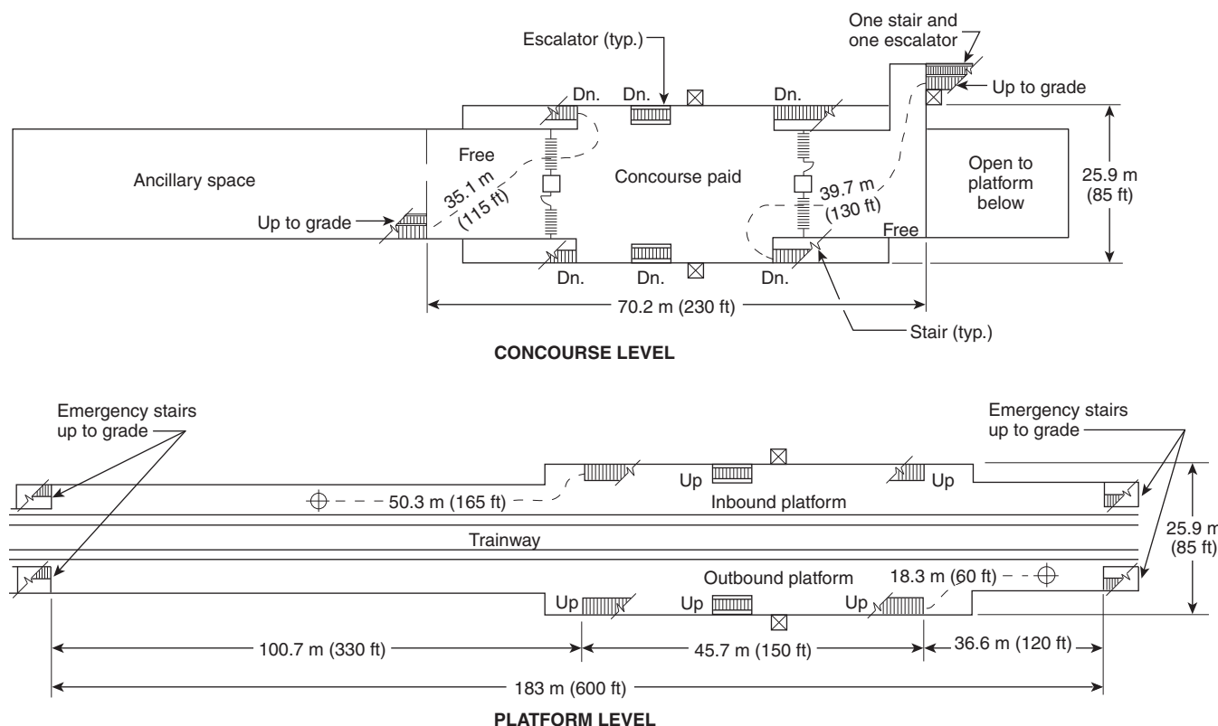
FIGURE C.1.4 Side-Platform Station.
